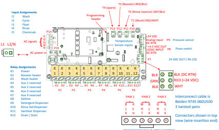
CONNECTING CONNECTOR TO DISPLAY PCB PN 05945-004-36-33
