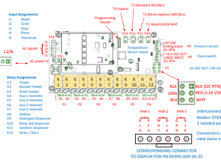
Connection Diagram for ID Module PN 02945-004-36-34
