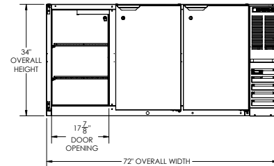
ELEVATION VIEW
