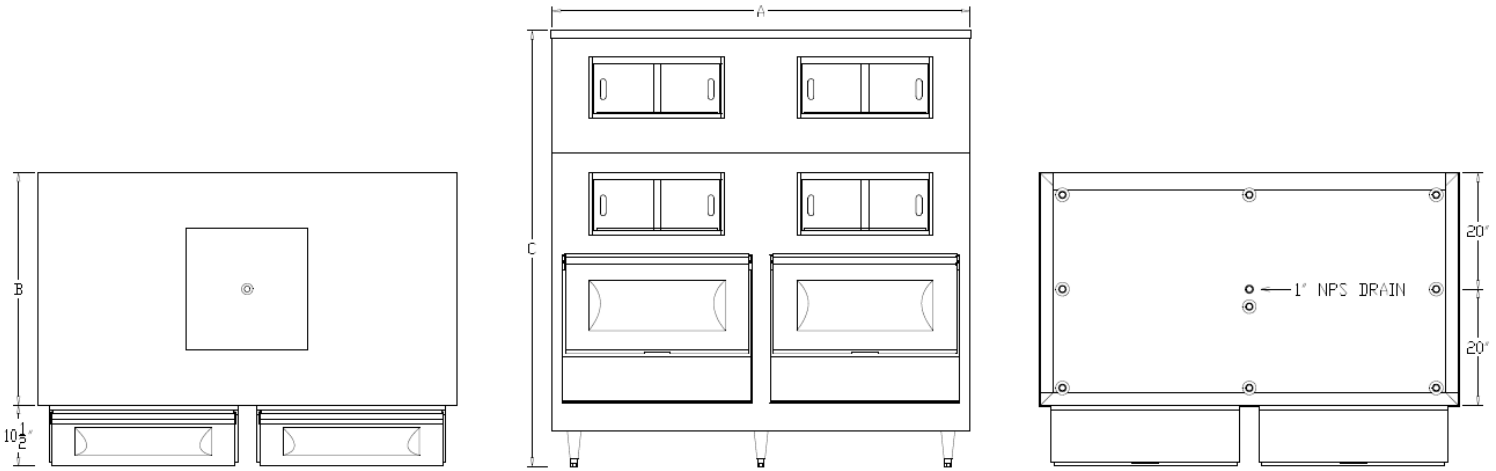
TOP VIEW
