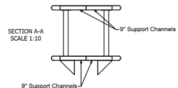
MAXIMUM WALL THICKNESS - 8"
