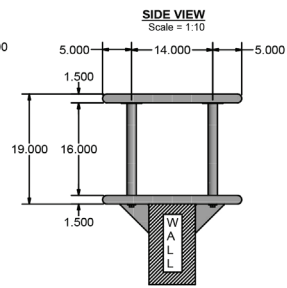
MAXIMUM WALL THICKNESS - 8"
