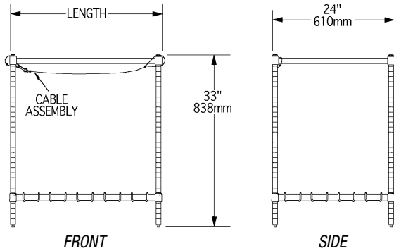
Style "A" Tank Racks
