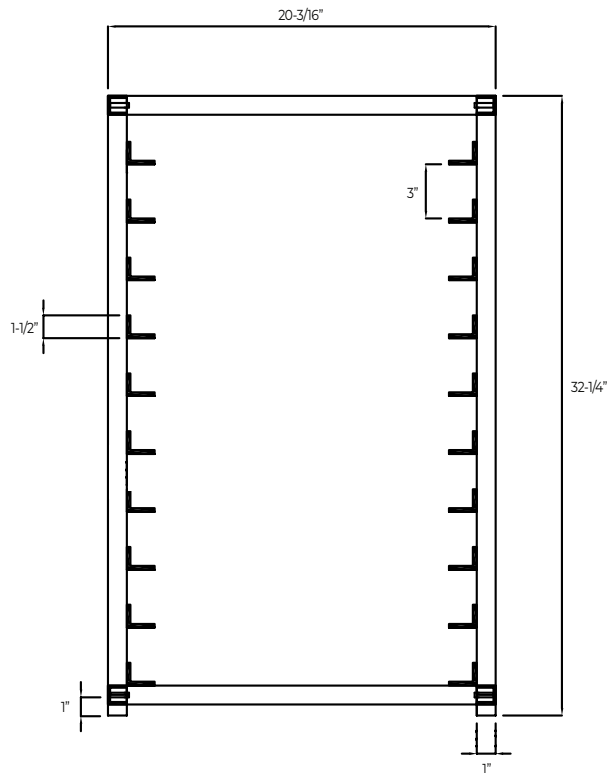
Front View
