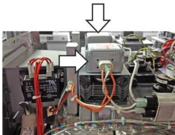
The 2000W e2s variant comprises two magnetrons located on the left and right hand sides of the cooling duct.
