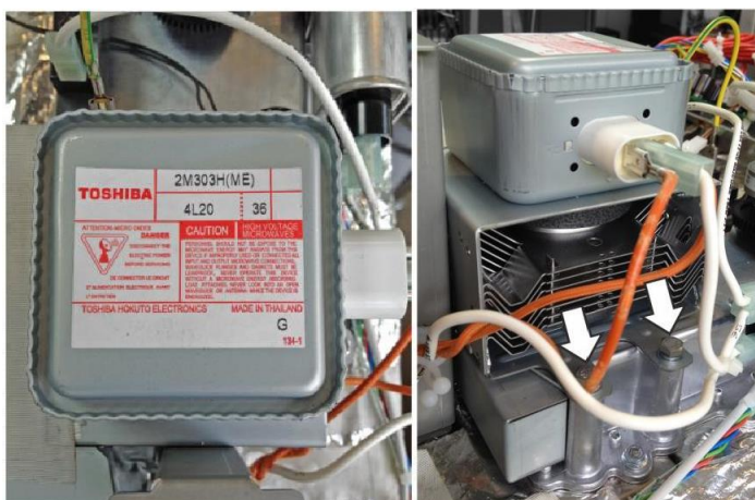
The magnetron(s) is/are located on top of the cavity and is/are fixed to the cooling duct and the cavity roof.
