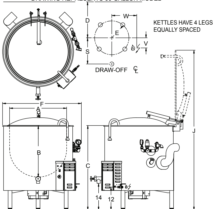
DRAWING REPRESENTS 60 GALLON MODEL
