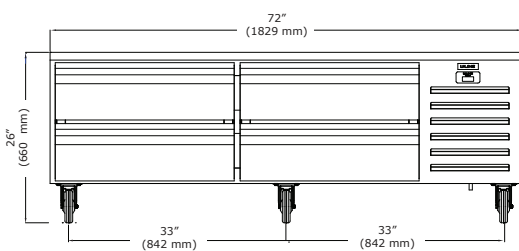
Front (72" Model)
