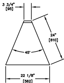
TSF45F-O
