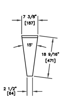
TS15F-I
