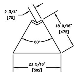
TS60F-O
