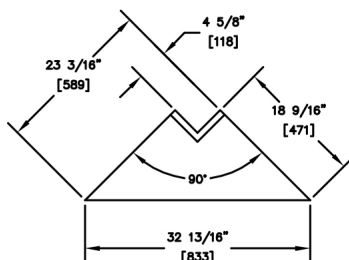
TS90F-O
