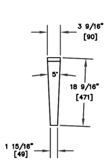
TS05F-I
