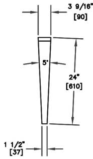
TSF05F-I
