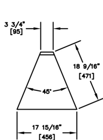
TS45F-O
