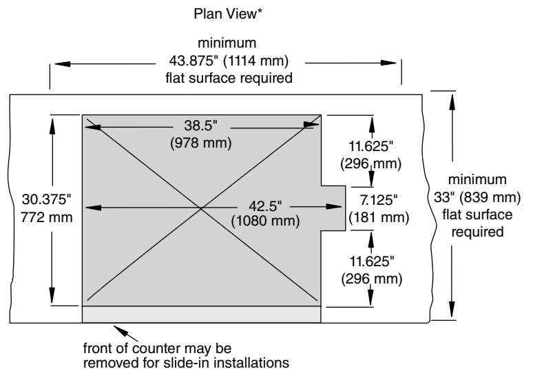
VUD300 series (dual-sided dispensing) drop-in installation
