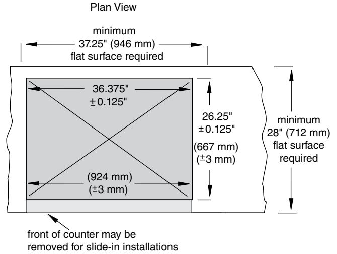
VU155 series with 10 valves drop-in installation
