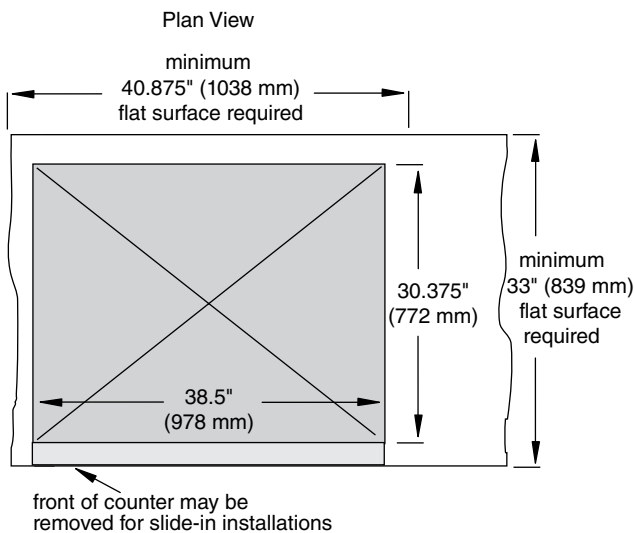
VU300 and CVU300 series drop-in installation
