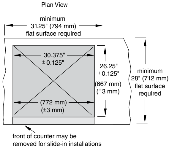
VU155N and VU155 series with 8 valves and CVU155N series drop-in installation
