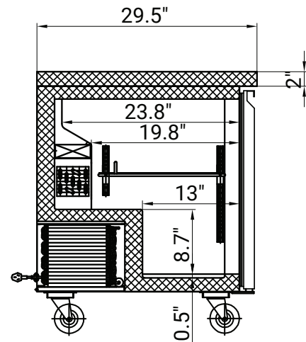
SECTION VIEW
