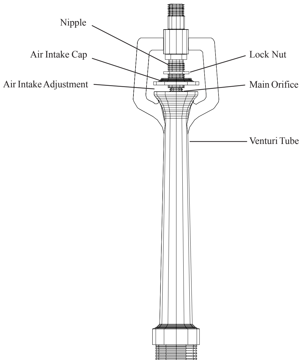
Venturi Assembly
