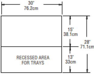
PLAN VIEW KCTS-28
