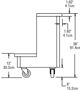
END VIEW KCTS-28
