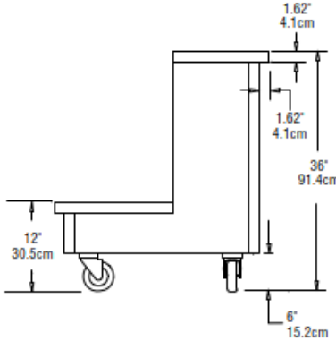
END VIEW KCTS-36
