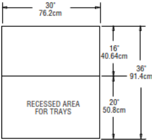
PLAN VIEW KCTS-36
