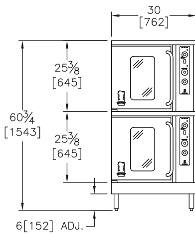
FRONT VIEW 2EK8(N)A WITH MODULAR BASE
