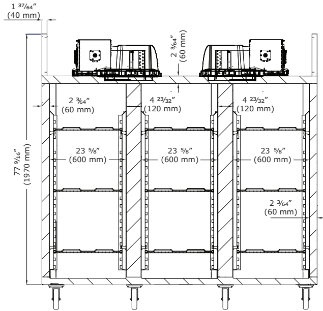
Front (Open)
