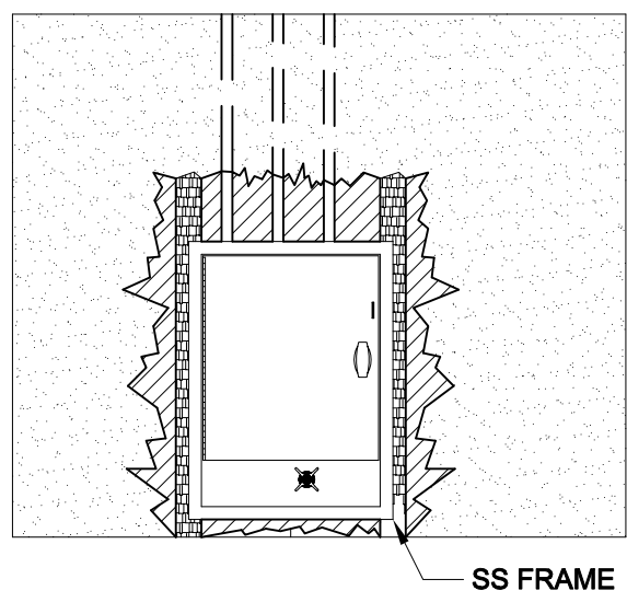
RECESSED MOUNTING
