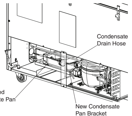
Condensate Pan Bracket Condensate Drain Hose
