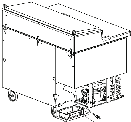
New Condensate Pan Bracket New Heated Condensate Pan
