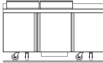
ST4472NP-12 Elevation View
