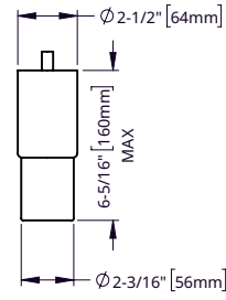
LEG DETAIL
