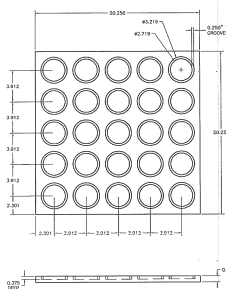
CUP SIZE: 3.02" DIA.
