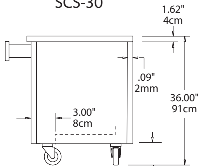
End View SCS-30
