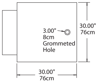
Plan View SCS-30
