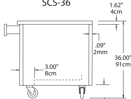
End View SCS-36
