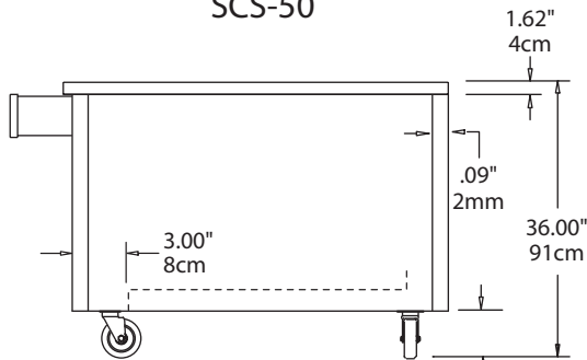
End View SCS-50
