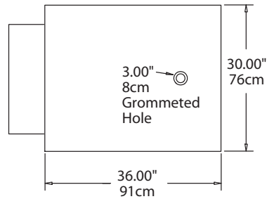
Plan View SCS-36
