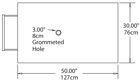
Plan View SCS-50
