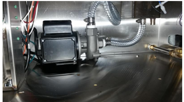
Wash pump with rinse pump removed
