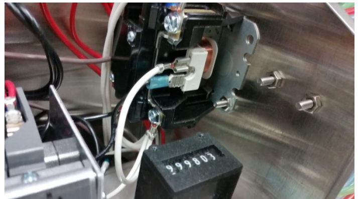
Wash motor contactor next to rack counter
