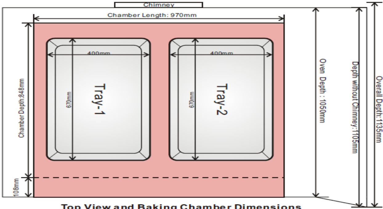
Top View and Baking Chamber Dimensions
