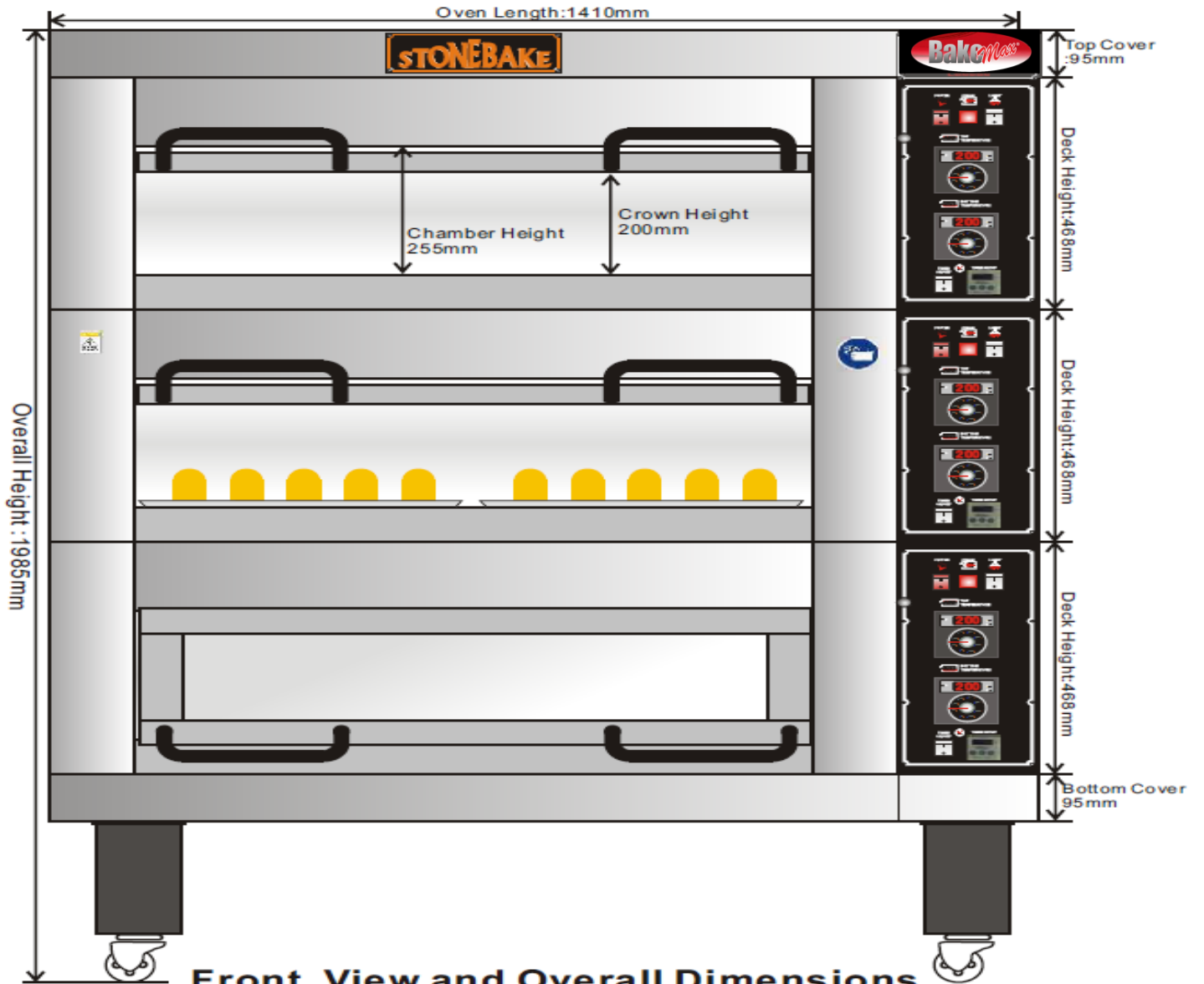
Front View and Overall Dimensions
