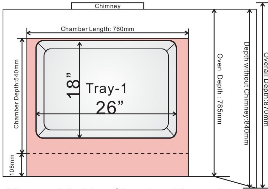
Top View and Baking Chamber Dimensions
