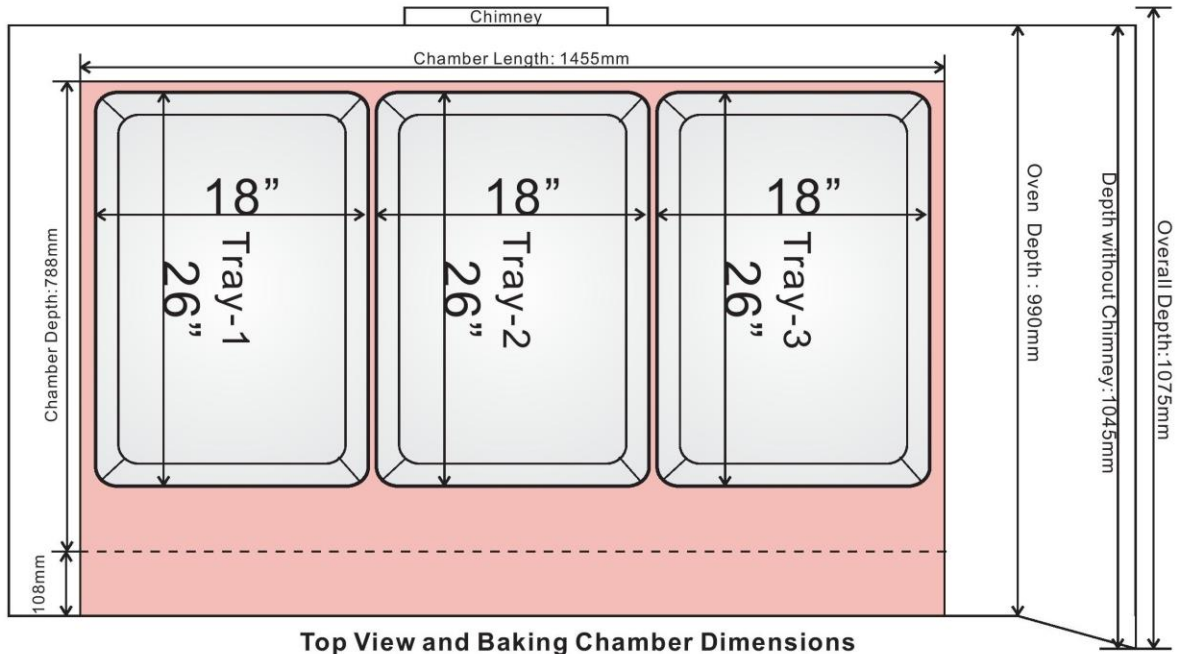
Top View and Baking Chamber Dimensions
