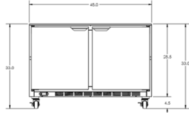
00A31-051A KIT - CASTER 3" WHEEL 3.75" HEIGHT 500 LB 401-633A / 401-634A 00A31-031D-03 LEVELER
