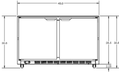
00C31-049A 2 3/4" CASTERS - "LOW PROFILE" 401-926D-01 / 401-926D-02
