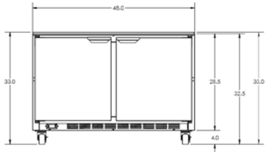
00A31-052A KIT - CASTER SPE/WT, 34" CUTTING BRD HEIGHT (UC 33") 3" CASTERS / 500# 401-695A / 401-696A 00C31-032D-03 LEVELER
