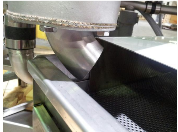
Correct alignment for sump to box
