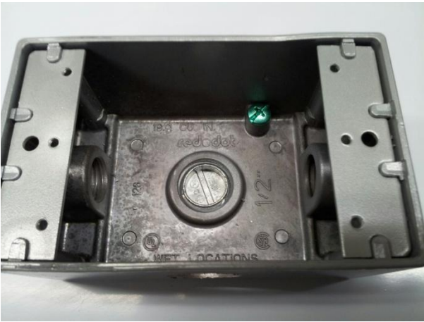
Inside view of the junction box w/green ground screw
