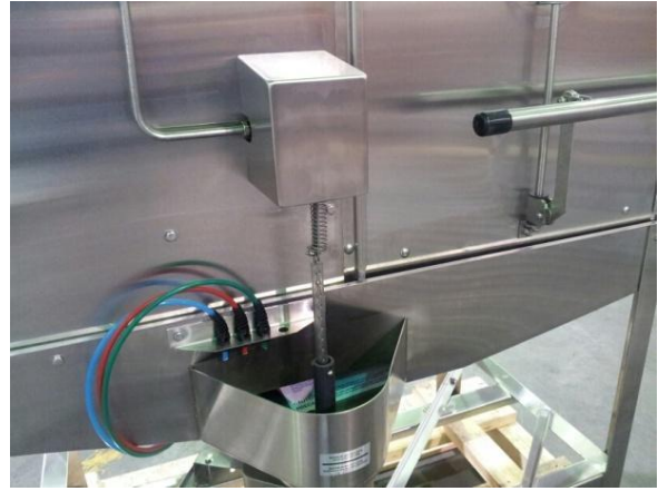
5-CD-RF Drain ball, sump, chemical feed lines
