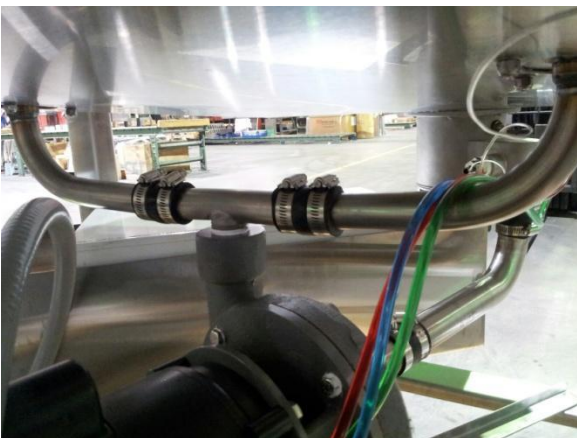
Pump discharge split/manifold
