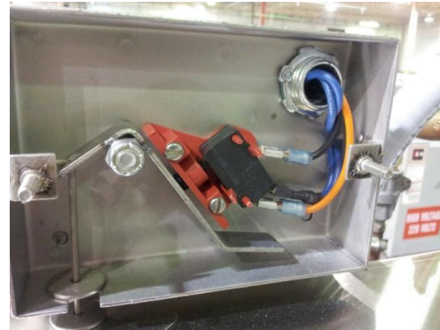
Showing "float" switch that controls fill water &amp; heater
