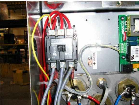
Showing booster contactor, yellow signal wire Copyright ADS Installation Manual Model HT-25 (4 wire), Revision 3.1, 6/14/2017
