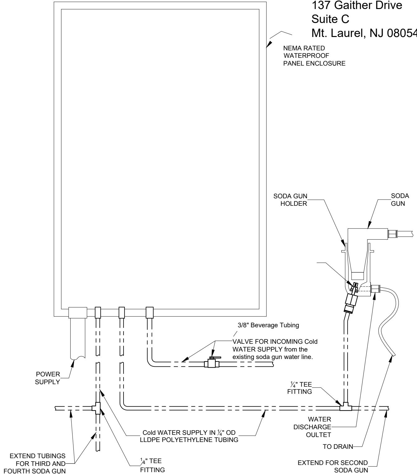
PLUMBING SCHEMATIC DIAGRAM - SODA/BAR GUN CLEANER (TYP FOR 4 SODA GUNS)
