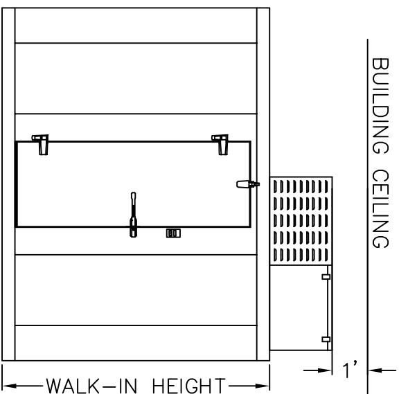
VIEW - A-
