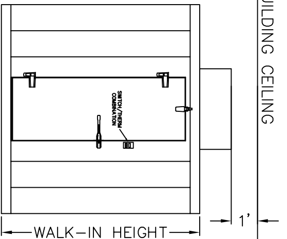
VIEW -A-
