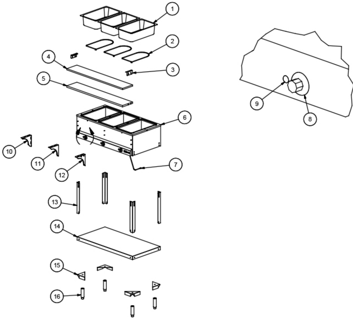
EXPLODED VIEW PARTS LIST
