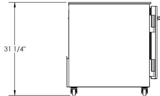
2 3/4" CASTERS
