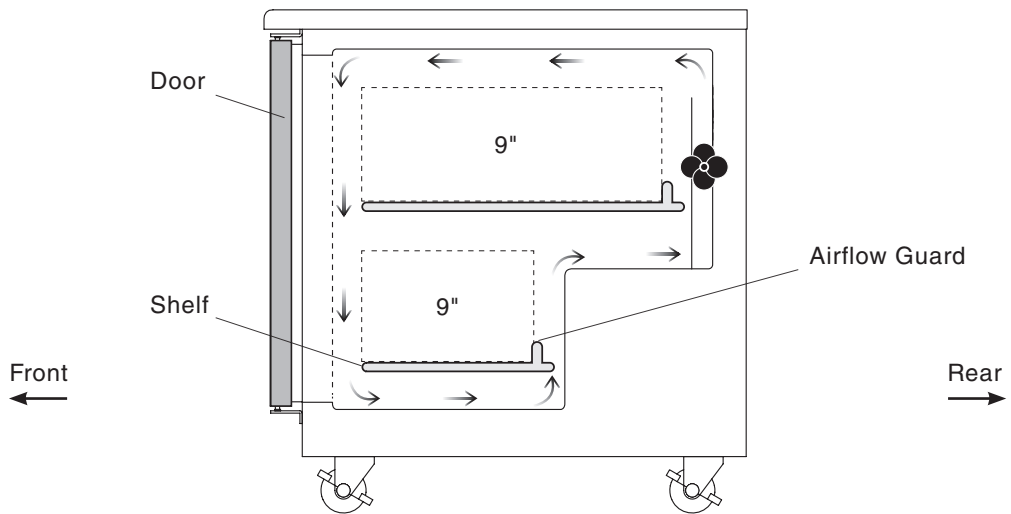
Side View
