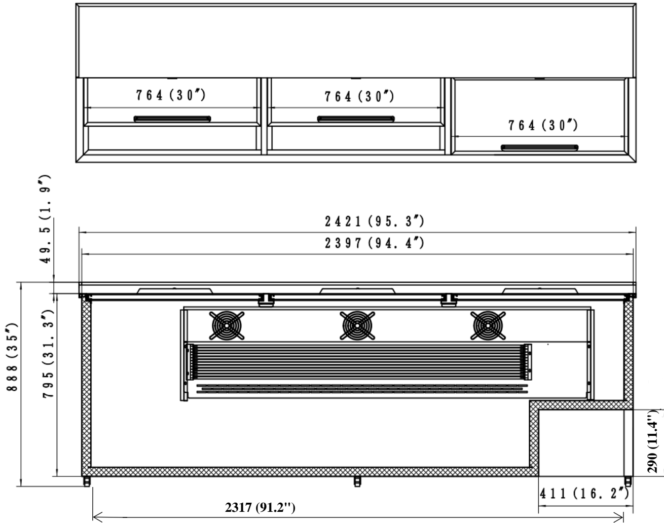
Dimensional Drawing VPB95
