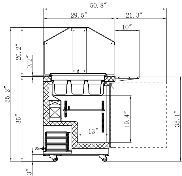
SECTION VIEW
