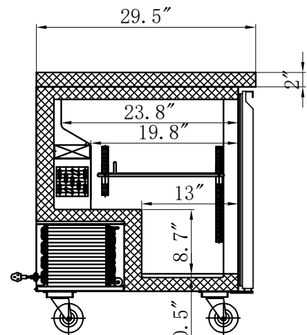
SECTION VIEW
