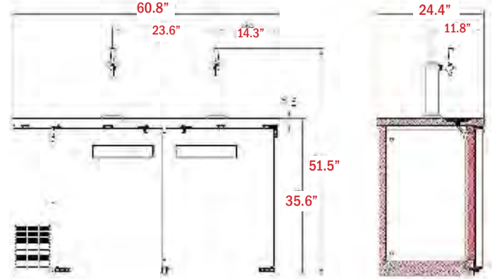
USBD-6024/2
