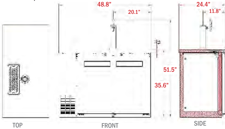
USBD-4824/2
