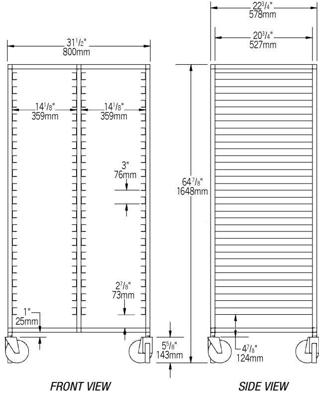
#OUR-1236-3-SR —Double-Width
