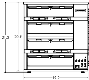
MHG42 with timer bars
