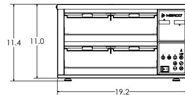
MHG22 without timers
