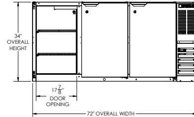
ELEVATION VIEW
