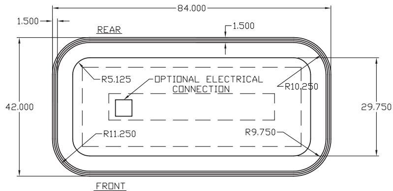
Plan View OD42I-7-LED
