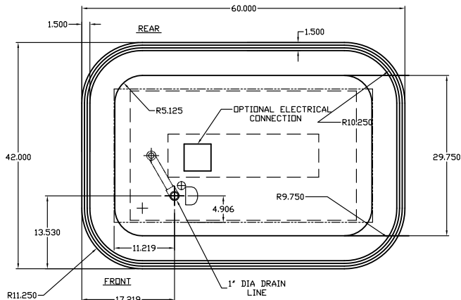
Self-Contained
