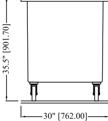
RANFG SW-8PS (END VIEW)
