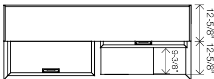
FBC-65(S)-HC Top View
