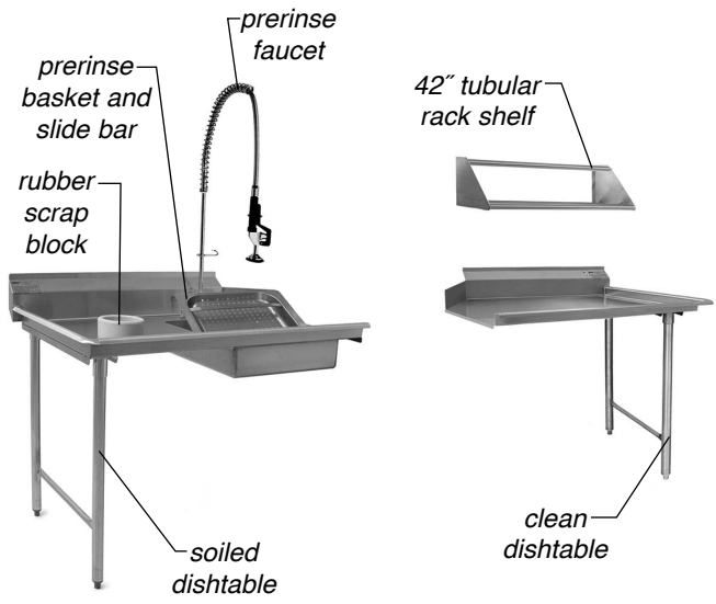
#DTC-48-LR-16/3 left-to-right operation shown
