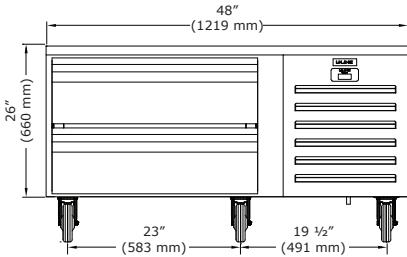
Front (48" Model)
