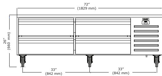
Front (72" Model)
