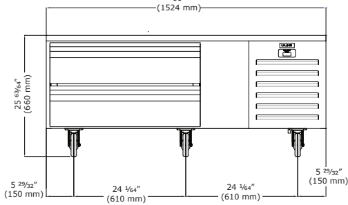
Front (60" Model)
