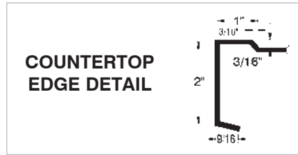
Countertop Edge On All Four Sides
