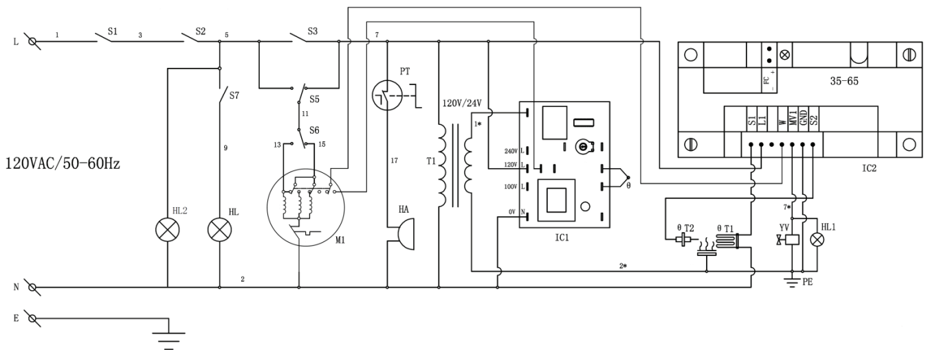
Wiring diagram
