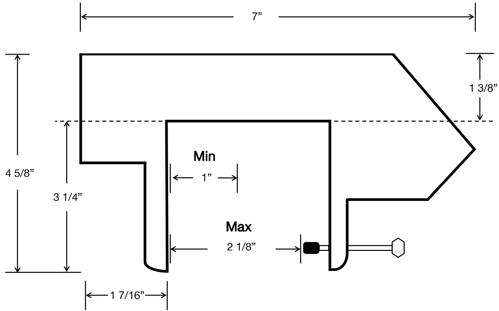
SIDE ELEVATION
